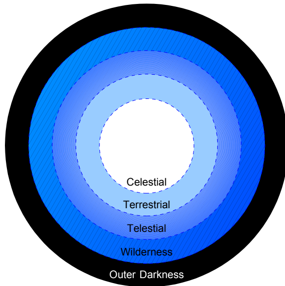
Proposed Cosmology
