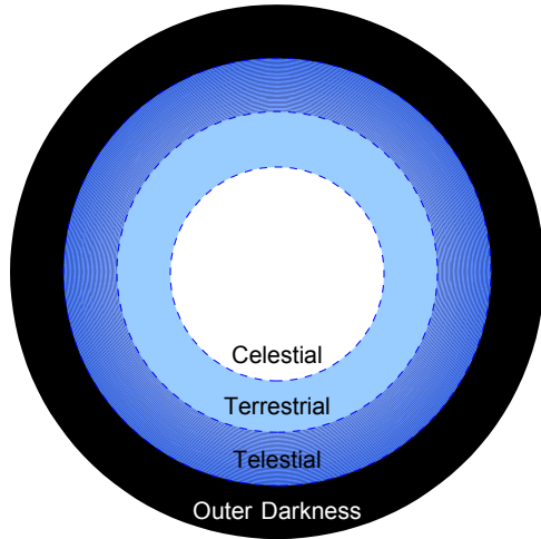
Traditional Cosmology
